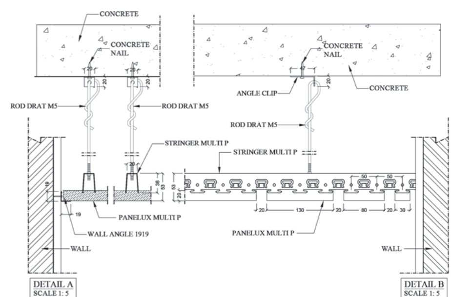
MULTI-P CEILING INSTALLATION
